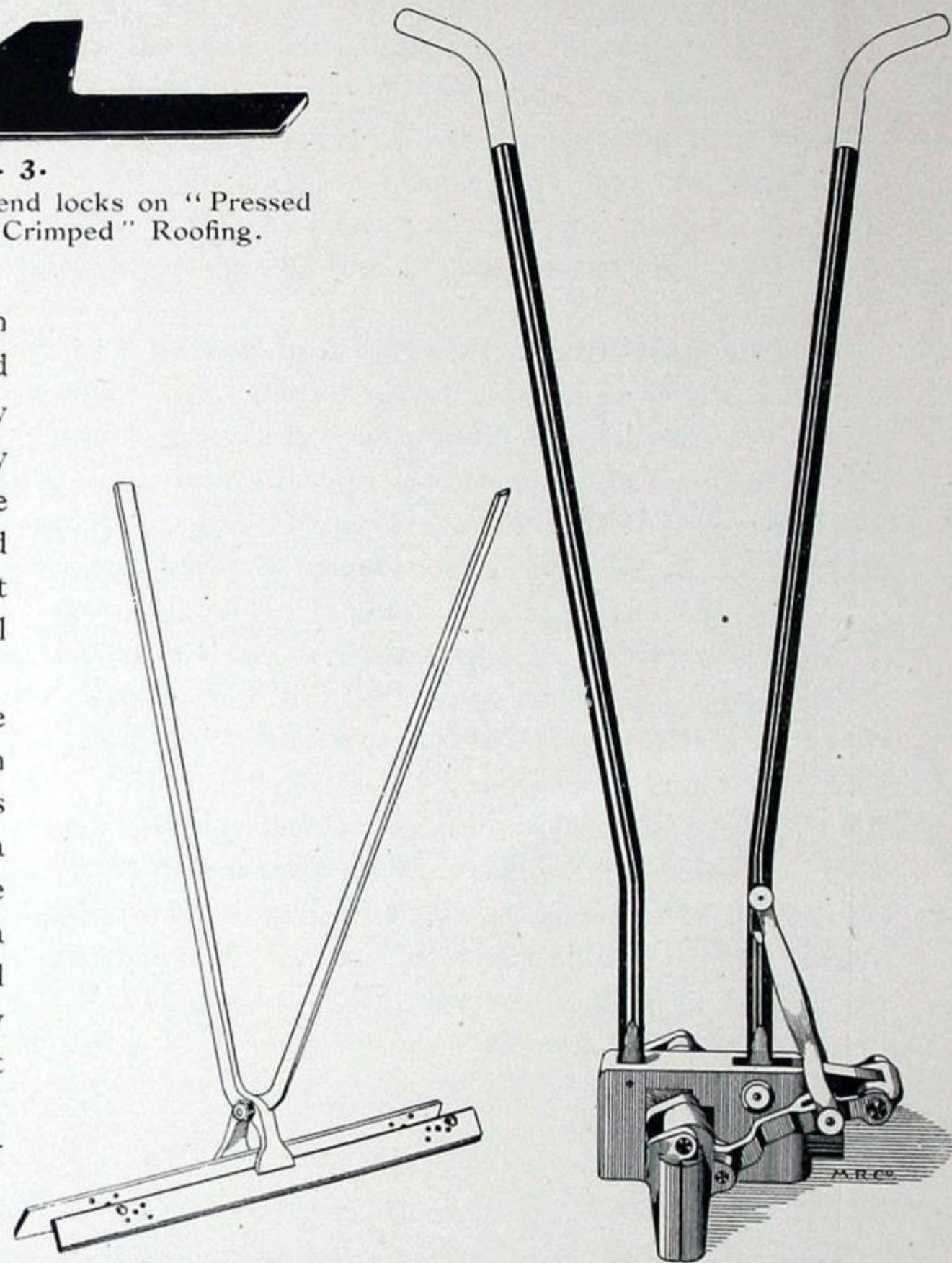
Fig. 4. Edging Tongs used with "Ready Roll Cap" Roofing, will turn seam 1, 1 1/4 or 1 1/2 inches high.
